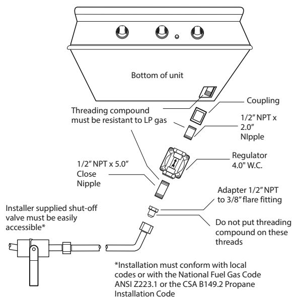
FIG. 07 Natural Gas
