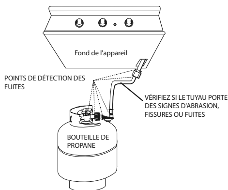
FIG. 15 Gaz propane
