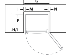
2. Flush with refrigerator door – full door rotation
